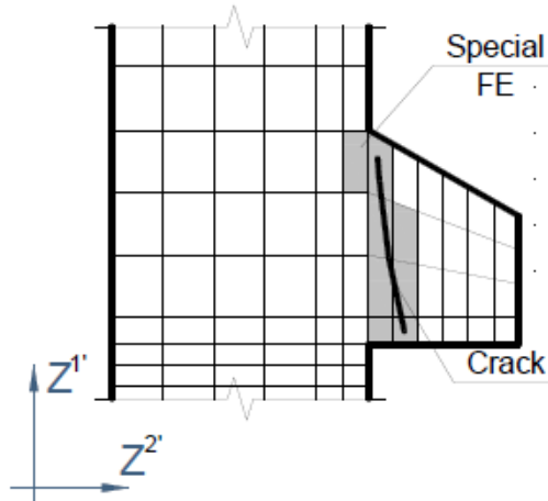
Fig. 3. Fragment of a FEM with special finite elements with cracks
