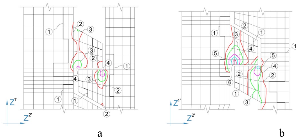
Fig. 2. The intensity of plastic deformations in section I-I: a – in the zone of the third projection; b – in the zone of the first projection
